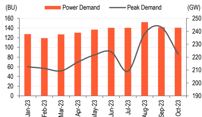
Fig 3 – Monthly peak power demand
