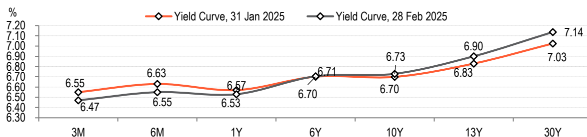
Figure 1: Movement in India's yield curve
